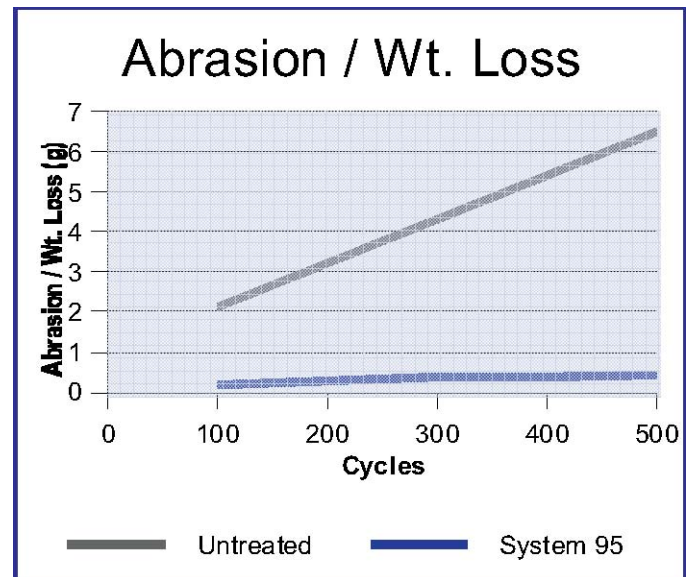
Figure: Loss in weight by Taber Abraser, Treated vs. Untreated Sandstone, at number of Cycles Indicated
